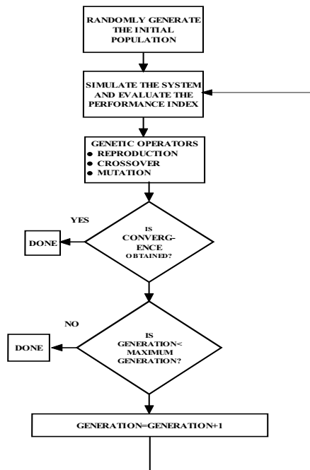
Fig. 1 Flow chart of genetic algorithm
