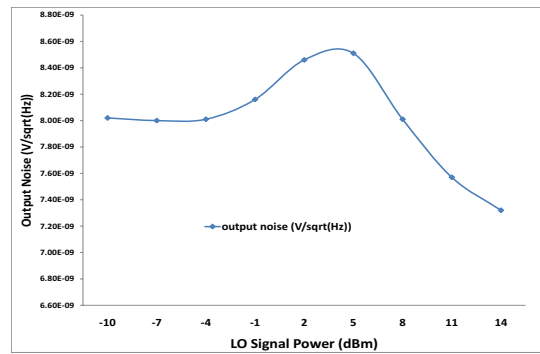
Fig. 7. Total amount of noise in nV/\sqrt{Hz} at the mixer output
