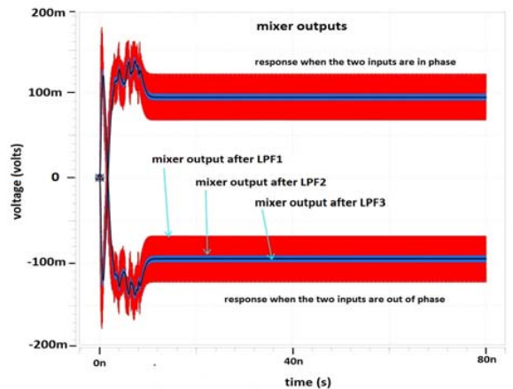
Fig. 12. Outputs of the mixer after different stages of the LPF
