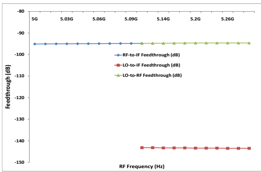
Fig. 5. Port-to-port isolation parameters for the RF multiplier
