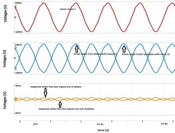
Fig. 11. Zero IF response when mixer inputs have two phase shifted combinations
