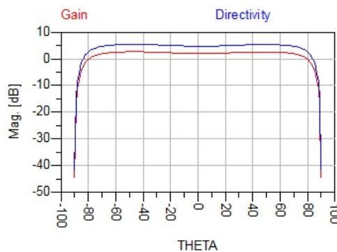
Fig. 6 Gain and directivity for 2.6 GHz
