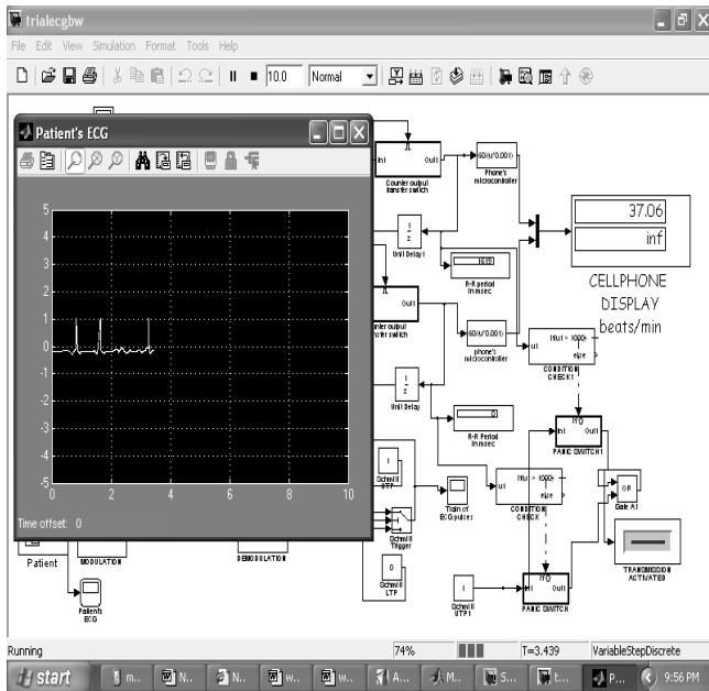
Fig. 6 Simulation of WET and Mobile ECG Analyzer
