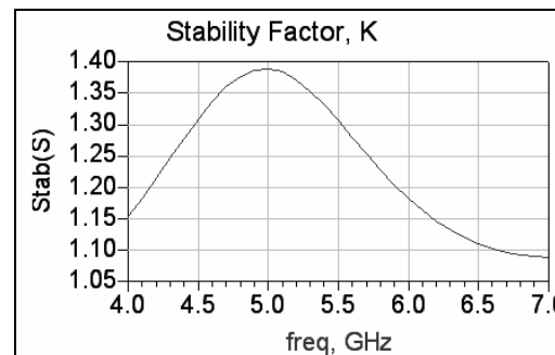
Fig. 11 Stability Factor (K) Plot
