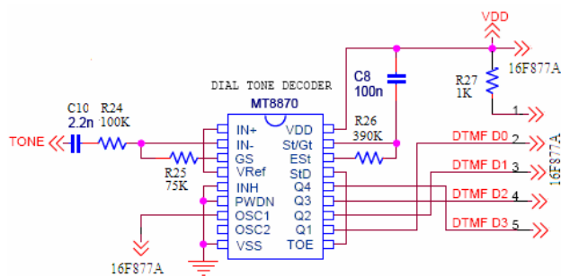
Fig. 9 Connection between Microcontroller System and DTMF
