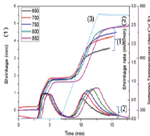
Fig. 2 Sintering profile of sintered samples
