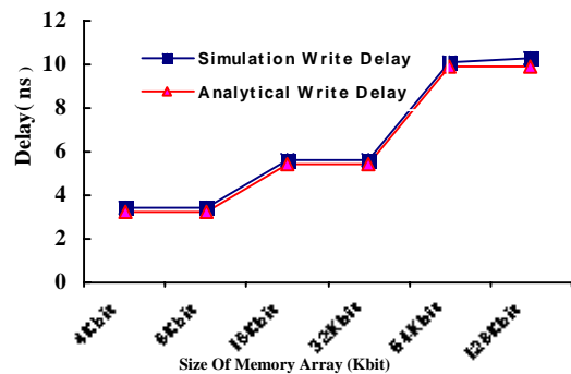
Fig. 7 Simulation and analytical write delay
