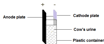
Fig. 2 Schematic representation of a single bio-voltaic cell
