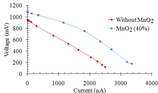
Fig. 4 Current-Voltage (I-V) characteristics of cow's urine battery and customized cow's urine battery
