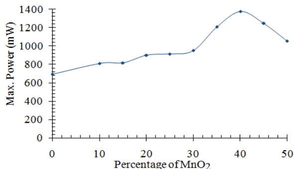
Fig. 3 Maximum power of varying percentage of \text{MnO}_2 (by weight) effect of performance with cow's urine
