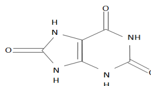
Fig. 1 The structure of uric acid [3], [7]
