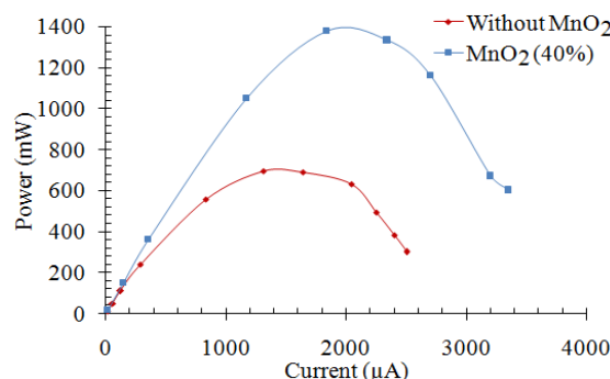
Fig. 5 Current-Power (I-P) characteristics of cow's urine battery and customized cow's urine battery
