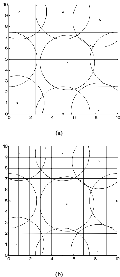
Fig. 1 Grid based coverage estimation for 9 sensors with sensing range equal to 2.5 in ROI of 10x10.(a) Grid size: 2.5x2.5; coverage estimated: 100% (b) Grid size: 1x1; coverage estimated: 95%
