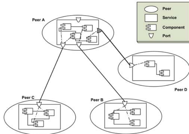
Fig. 2. Service Composition Example.
