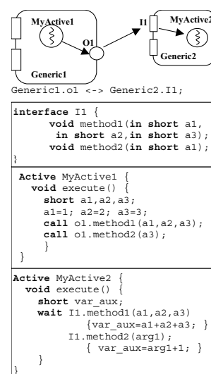
Fig. 1. Synchronization Primitives.
