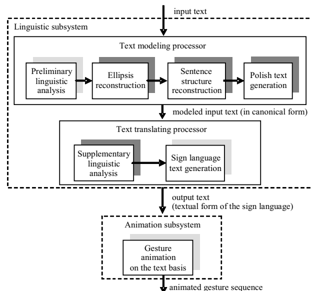
FIG. 1. TRANSLATION SCHEME IN THE THETOS SYSTEM (DARK-SHADOWED BLOCKS DID NOT APPEAR IN THE PRIMARY VERSION)
