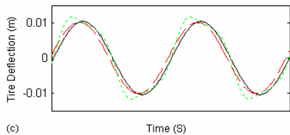
Fig. 5 Steady state analysis of 4DOF model ( \omega=4 HZ) a) Body acceleration b) Roll angle c) Tire deflection
