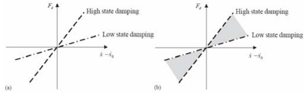
Fig. 2 Semi-active damper concepts
