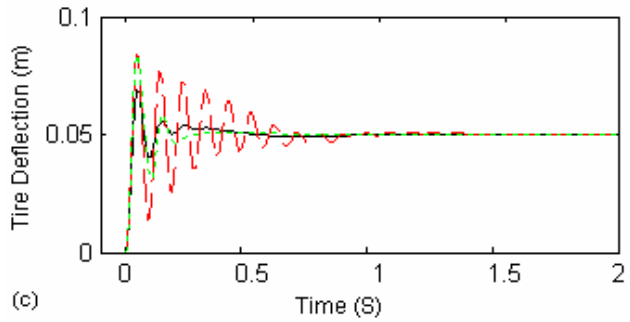
Fig. 4 Transient analysis of 4DOF model a) Body acceleration b) Roll angle c) Tire deflection
