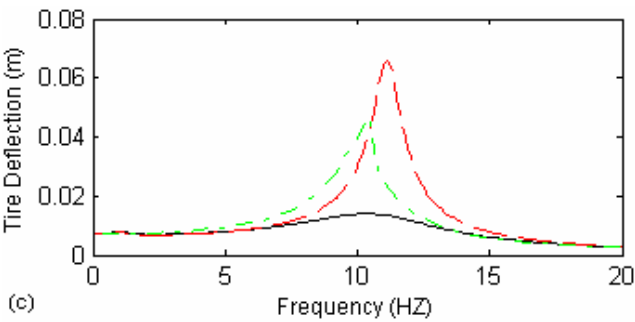
Fig. 3 Frequency analysis of 4DOF model a) Body acceleration b) Roll angle c) Tire deflection
