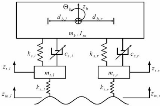
Fig. 1 Roll plane vehicle - model
