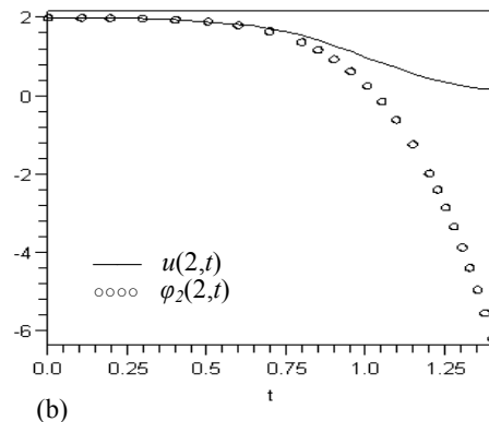
Fig. 3 Results for x=2 , obtained for the exact solution (solid line) and the ones obtained by applying PA [2/6] and [2/7] to \varphi_2 , shown in (a), in comparison with HPM result \varphi_2 , shown in (b), for cubic modified Boussinesq equation (18)
