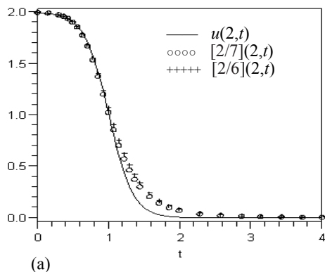
Fig. 3 Results for x=2 , obtained for the exact solution (solid line) and the ones obtained by applying PA [2/6] and [2/7] to \varphi_2 , shown in (a), in comparison with HPM result \varphi_2 , shown in (b), for cubic modified Boussinesq equation (18)
