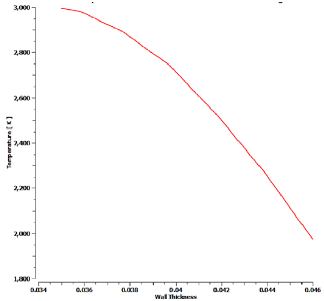
Fig. 4 Temperature variation in combustion chamber wall without cooling
