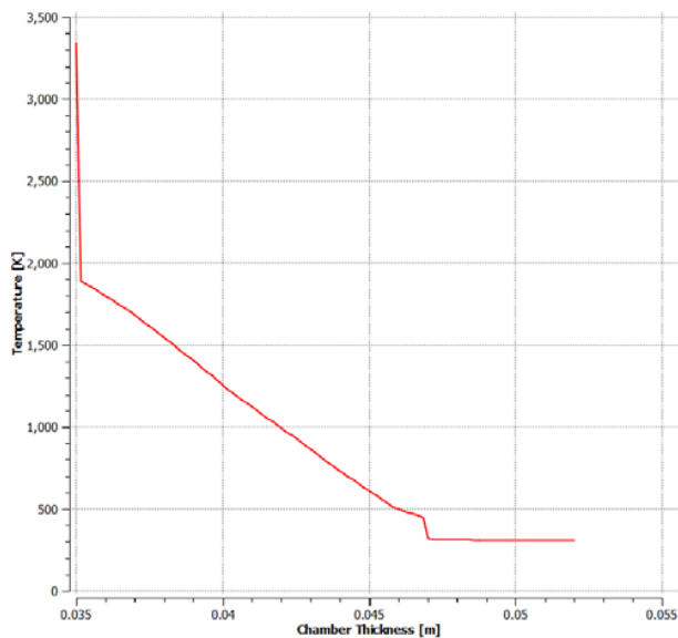
Fig. 6 Temperature variation in combustion chamber after cooling
