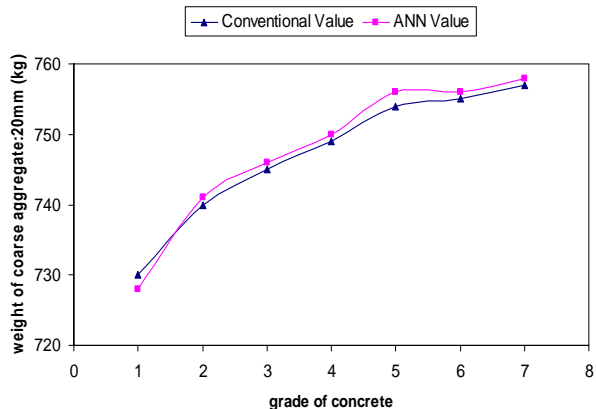
Fig. 5 Comparison of 20 mm coarse aggregate/weight per meter cubic concrete for various mix grades
