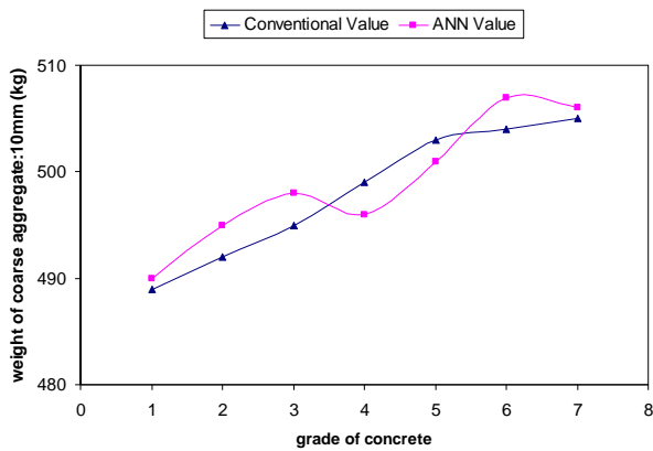
Fig. 2 Comparison of cement/weight per meter cubic concrete for various mix grades
