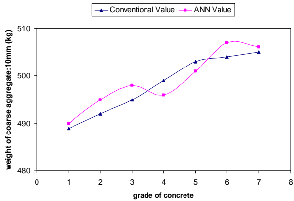
Fig. 4 Comparison of 10 mm coarse aggregate/weight per meter cubic concrete for various mix grades
