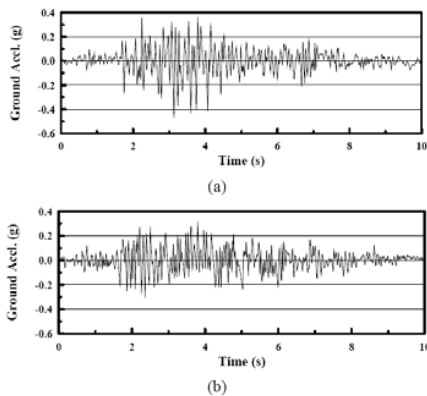
Fig. 6 Ground motion recorded at the Koyna Dam for the 1967 Koyna earthquake: (a) the stream component; (b) the vertical component
