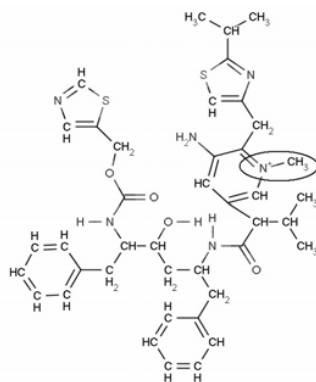
Fig. 5 Structure of Ritonavir Analog 11
