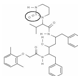
Fig. 3 Structure of Lopinavir Analog 8
