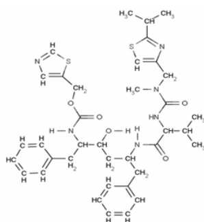
Fig. 4 Structure of Ritonavir
