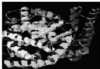
Fig. 1 Structure of ACE-2
