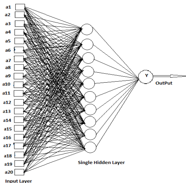
Fig. 4 Constructed Neural Network Architecture.
