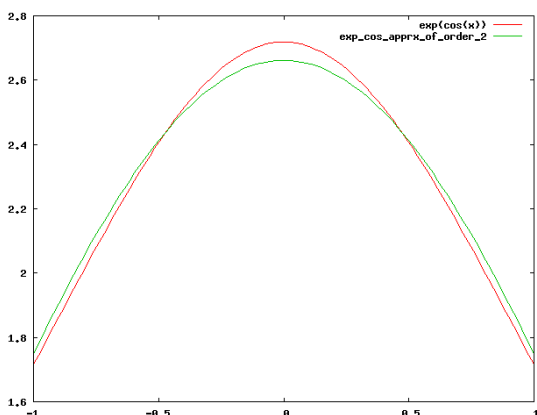
Fig. 7. Approximating \exp(\cos(x)) using Chebyshev
