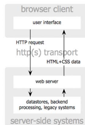
Fig. 1 Client-Server Architecture [1]
