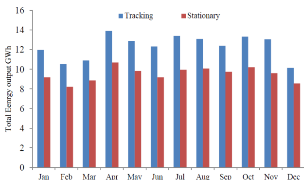
Fig. 3 Monthly total energy output for both stationary and tracking systems
