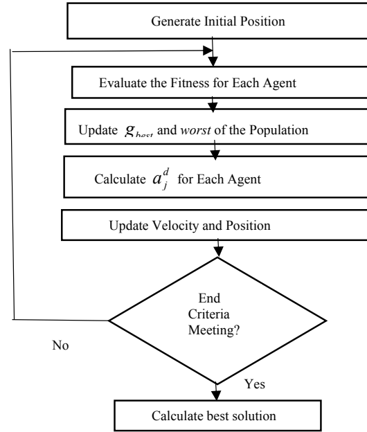
Fig. 2 Flow Chart of Gravitational Search Algorithm
