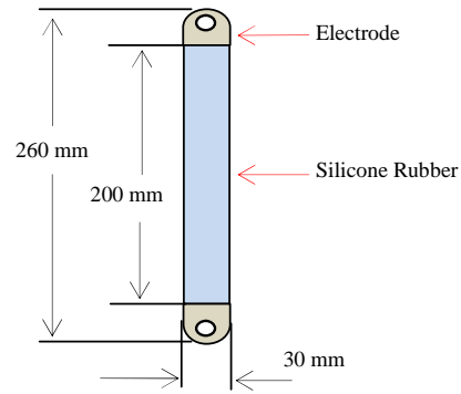
(a) Salt fog ageing test
