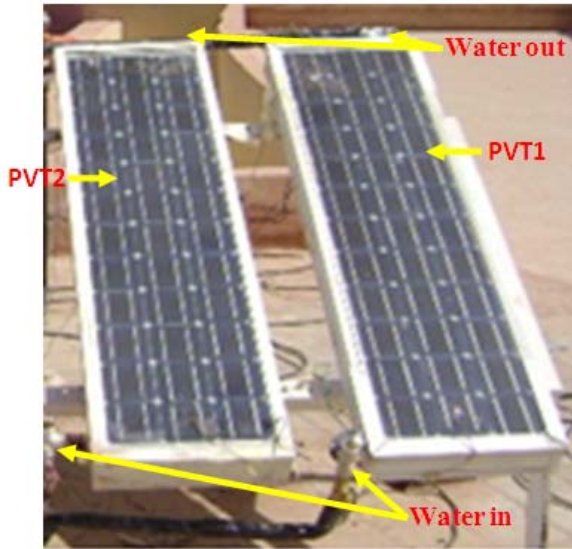
Fig. 3 Test bench mounted unit URAER
