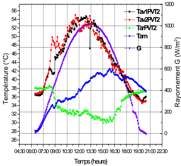
Fig. 5 Temperatures of PVT 2
