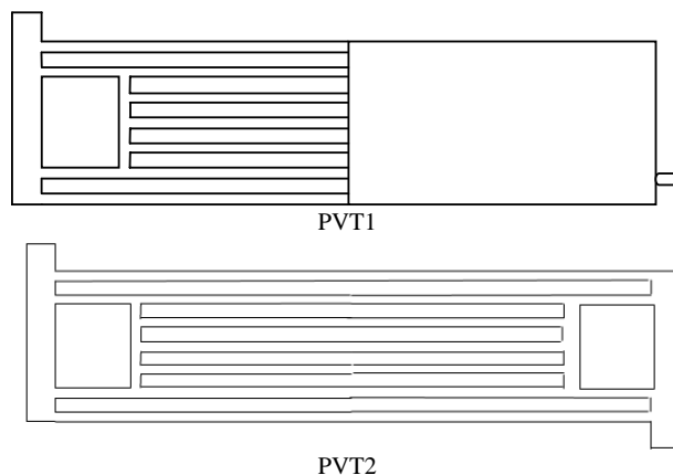
Fig. 1 Both configurations of hybrid collectors
