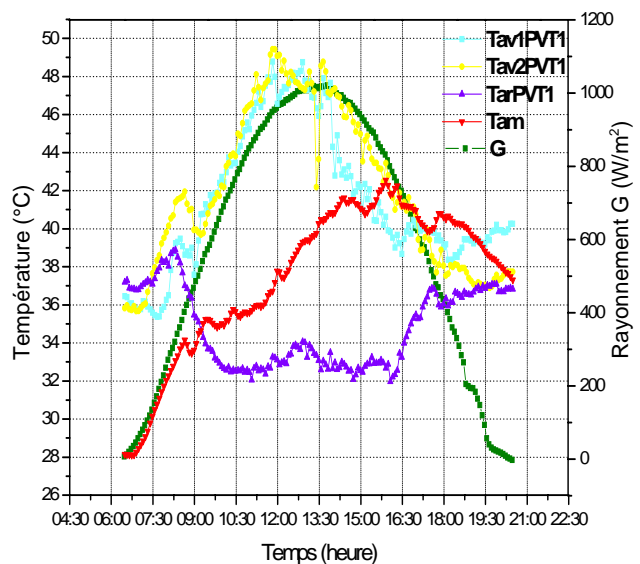
Fig. 4 Temperatures of PVT 1
