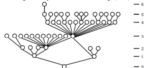
Fig. 10 Graph Scheme before change (B=1)
