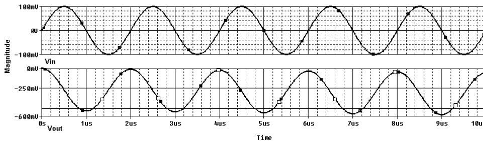
Fig. 16 Output waveform of the MOS-C Op-amp integrator
