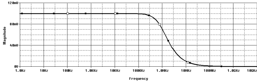
Fig. 21 Frequency response of OTRA based integrator
