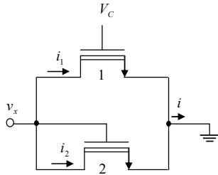
Fig. 7 Fourth nonlinear cancellation technique
