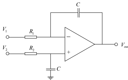
Fig. 14 Op-amp based integrator circuit
