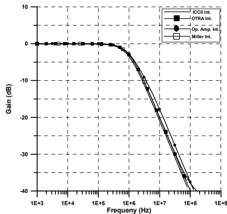
Fig. 26 Frequency responses of the four integrators
