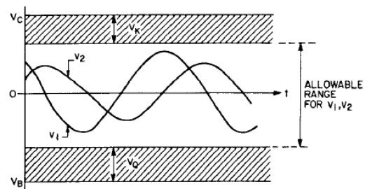
Fig. 2 Terminal voltages for the transistor [1]
