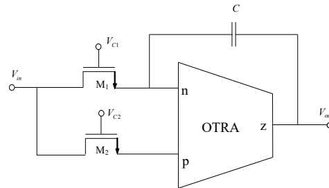
Fig. 19 MOS-C realization of OTRA based integrator
