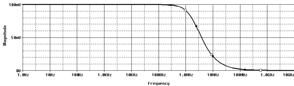
Fig. 25 Frequency response of ICCII based integrator
