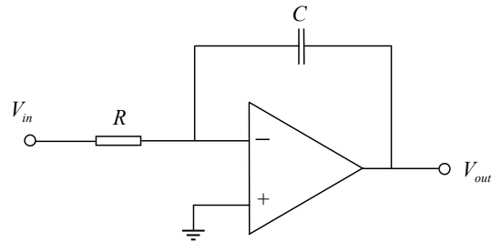
Fig. 8 Miller integrator
