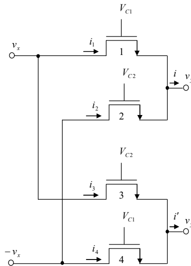
Fig. 6 Third nonlinearity cancellation technique
