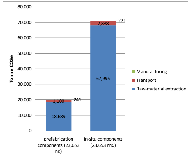
Fig. 13 The initial embodied carbon emission from the raw-material extraction to construction site for production of the 23,653 numbers of in-situ elements for a public housing development in Kai Tak area
