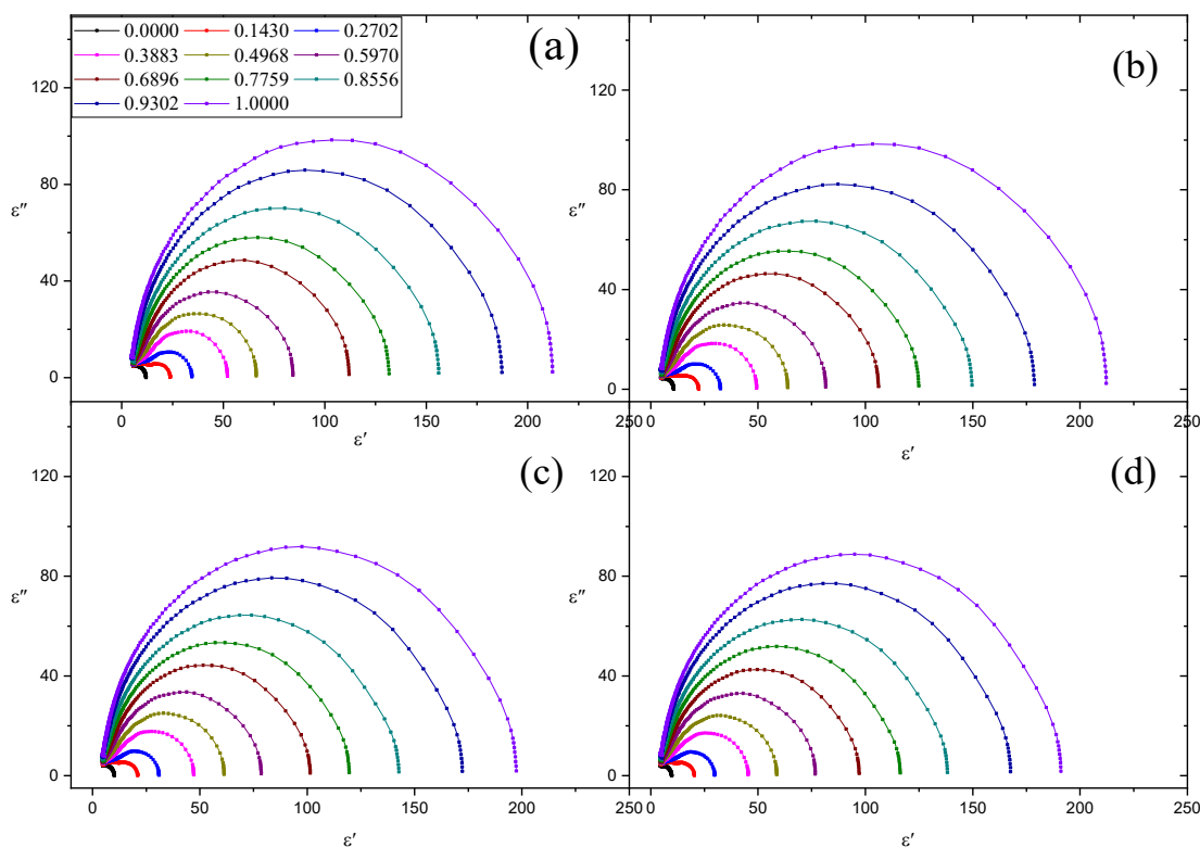
Fig. 4 Complex plane plot of dielectric constant ( \epsilon' ) vs. dielectric loss ( \epsilon'' ) for various concentrations of NMF in DE at (a) T = 10^\circ\text{C} , (b) T = 15^\circ\text{C} , (c) T = 20^\circ\text{C} , and (d) T = 25^\circ\text{C}
