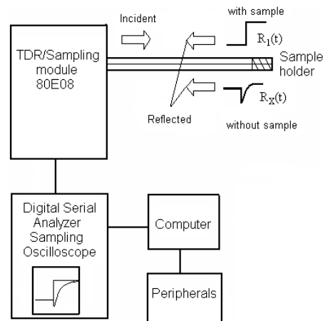
Fig. 1 Block diagram of TDR setup
