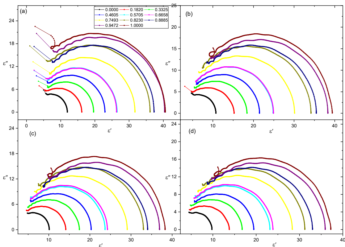
Fig. 5 Complex plane plot of dielectric loss ( \epsilon'' ) vs. dielectric constant ( \epsilon' ) for various concentrations of DMF in DE at (a) T = 10\text{ }^{\circ}\text{C} , (b) T = 15\text{ }^{\circ}\text{C} , (c) T = 20\text{ }^{\circ}\text{C} , and (d) T = 25\text{ }^{\circ}\text{C}
