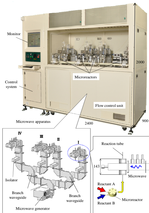
Fig. 9 Overview of Combined Microwaves and Microreactors Plant
