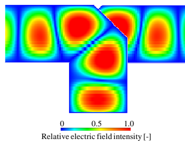
Fig. 4 Relative electric field intensity distribution
