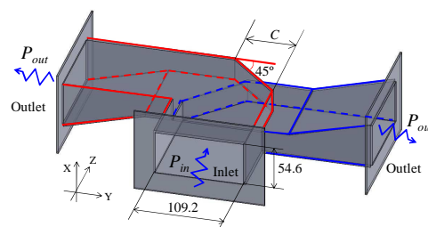
Fig. 2 Overview of branch waveguide (Model 2)
