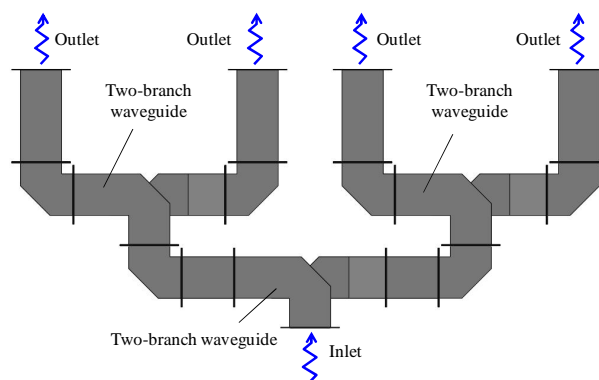
Fig. 6 Schematic of four-branch waveguide
