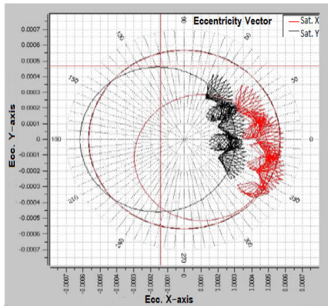
Fig. 7 Violation of the "Normal_vs_Radial separation" circle
