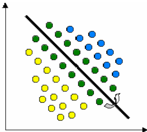
Fig. 2 Overlapping Clustering
