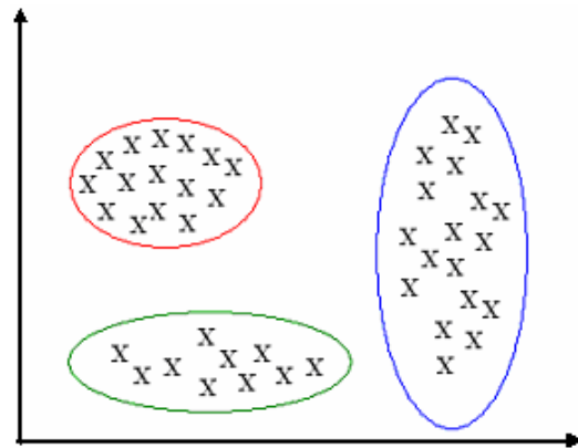
Fig. 1 Clustering
