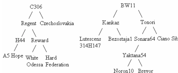
Fig. 3 Pedigree trees
