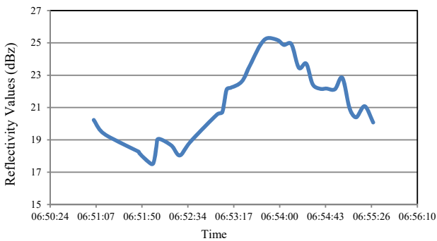
Fig. 4 Stratiform events on 28/8/2009 (Reflectivity Values)
