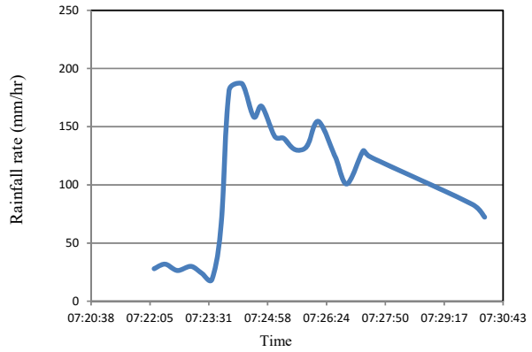
Fig. 5 Convective rain events on 05/08/2009 (Rainfall rates Values)
