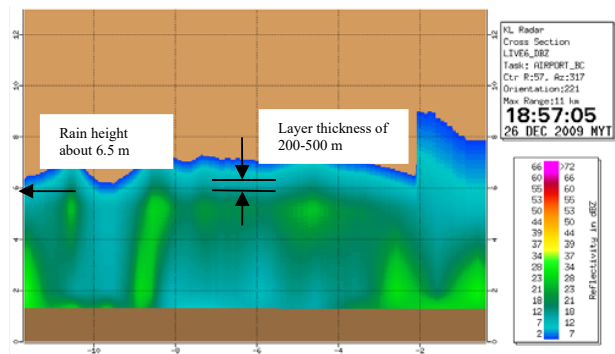
Fig. 7 Stratiform events on 26/12/2009
