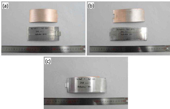
Fig. 3 Appearances of hot-rolled sheets processed by DSR at 150°C under the speed ratio of 2.1:1 with thickness reductions of 16.5% (a), 26% (b), and 27% (c), respectively
