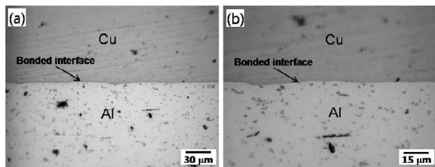
Fig. 5 Optical micrographs showing interface of clad sheet obtained at 100°C under the speed ratio of 2:1 with thickness reductions of 45%
