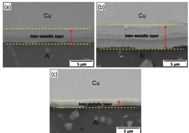
Fig. 6 SEM micrographs showing interface of clad sheet obtained at 100°C under the speed ratio of 2:1 with thickness reductions of 45% followed by annealing at 400°C for 30 (a), and 60 (b), and 120 min (c), respectively
