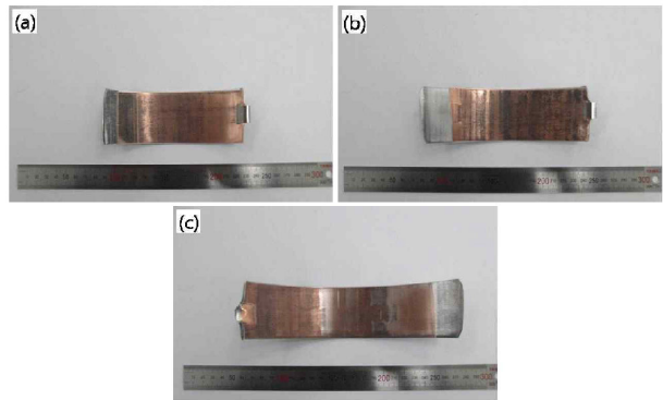
Fig. 4 Appearances of hot-rolled sheets processed by DSR at 100°C under the speed ratio of 2:1 with thickness reductions of 24% (a), 36% (b), and 45% (c), respectively
