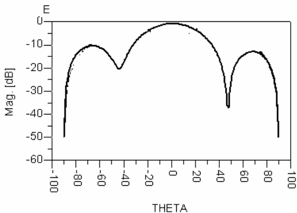
Fig. 7 The radiation pattern
