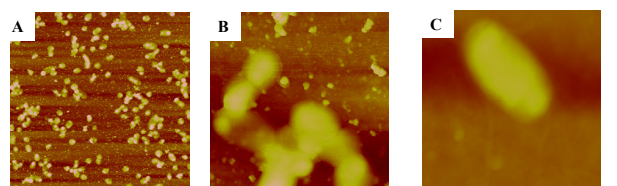
Fig. 7 AFM results obtained in tapping mode in air. Topography of bacteria immobilized on a surface functionalized by PAH-(PSS-PAH) 3 . Bacteria population (A: 30\mu\text{m} \times 30\mu\text{m} , B: 5\mu\text{m} \times 5\mu\text{m} ); an isolated bacterium (C: 3\mu\text{m} \times 3\mu\text{m} )
