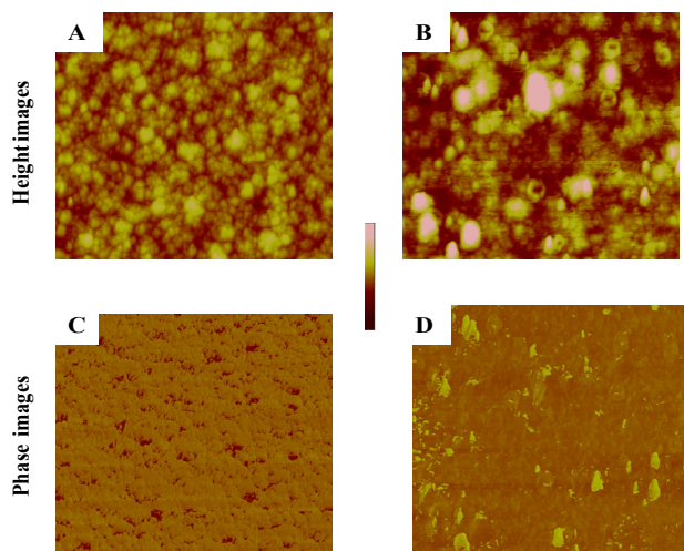
Fig. 6 Topographic images ( 5\mu\text{m} \times 5\mu\text{m} ) obtained in AFM tapping mode on bare surface (A and C, height and phase respectively), and on surface recovered with PEM (B and D, height and phase respectively). Scale bar for height and phase image are 50nm and 360^\circ , respectively
