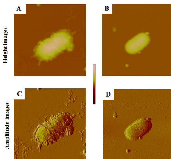
Fig. 8 AFM topography images ( 5\mu\text{m} \times 5\mu\text{m} ) obtained in tapping mode. Bacteria were incubated in a \text{SiO}_2 -NPs solution ( \Phi=100\text{nm} ) during 1 hour on mica substrate for two separate bacteria (A, C) and (B, D). Scale bar for height and amplitude images are 500 nm and 100mV, respectively
