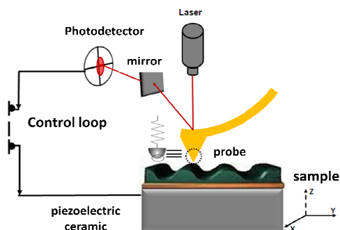
Fig. 3 Atomic Force Microscopy (AFM) principle
