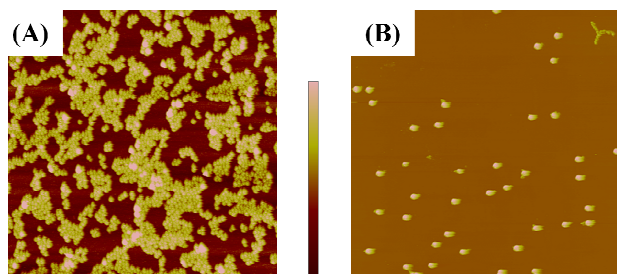
Fig. 4 AFM results on nanostructured surface with \text{SiO}_2 -NPs ( \Phi=100 nm). Amplitude images 10\mu\text{m} \times 10\mu\text{m} obtained with the tapping mode (A: dilution 500 \times , B: 1000 \times dilution)
