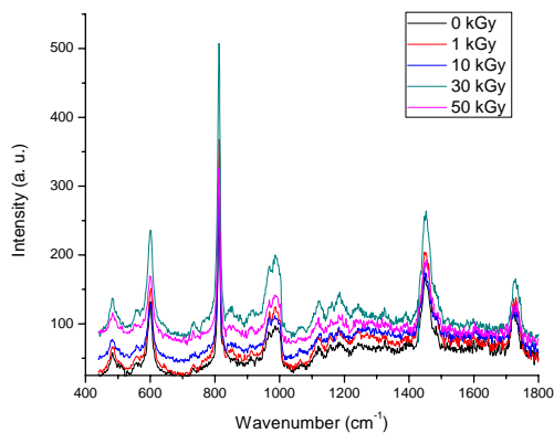
Fig 5 Raman spectroscopy acrylic resin, after curing, un-irradiated and irradiated
