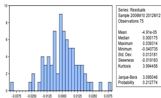
Fig. 3 Histogram of Residuals and Jarque-Bera Test Results
