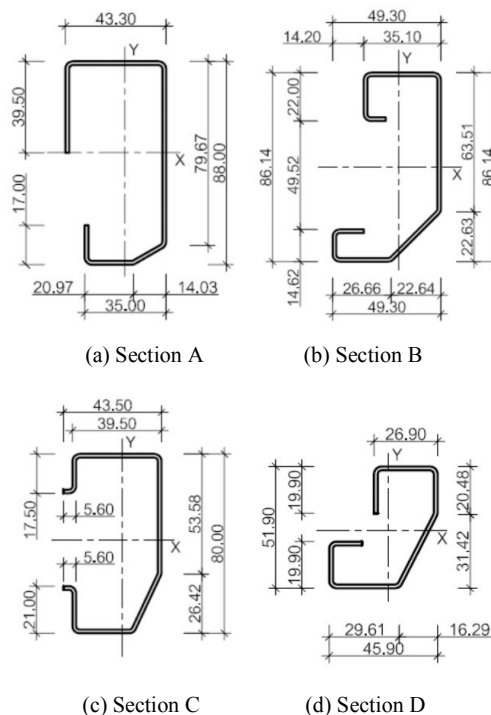
Fig. 2 Column sections (Unit: mm)
