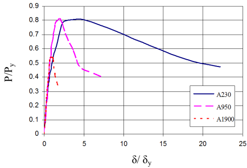
Fig. 9 P/P_y and \delta/\delta_y relationships of A-section columns
