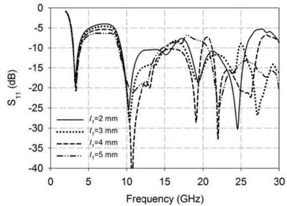
Fig. 2 Return losses versus frequency of the proposed antenna with: (a) varying \epsilon_r ; (b) varying R_d , varying R_s , and varying l_1
