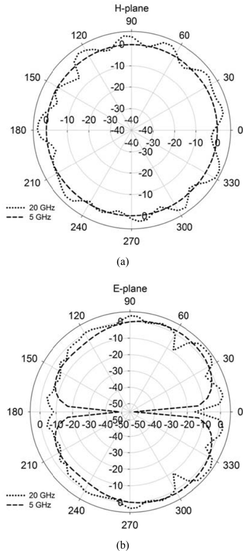
Fig. 4 Far-field radiation pattern of the proposed antenna: (a) H-plane; and (b) E-plane at 5 GHz and 20 GHz
