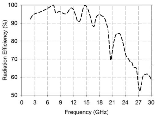
Fig. 5 Estimated radiation efficiency of the proposed antenna
