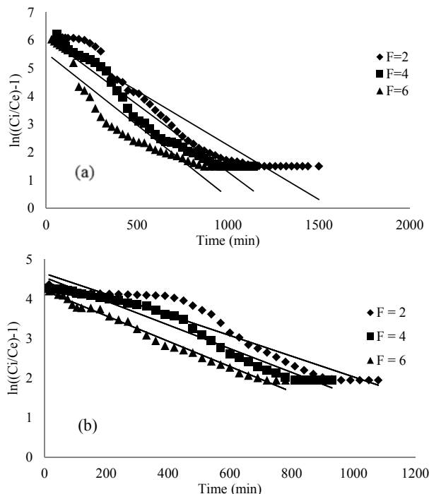
Fig. 4 Thomas model for biosorption of Cu (A) and Mn (B) ions at different flow rates
