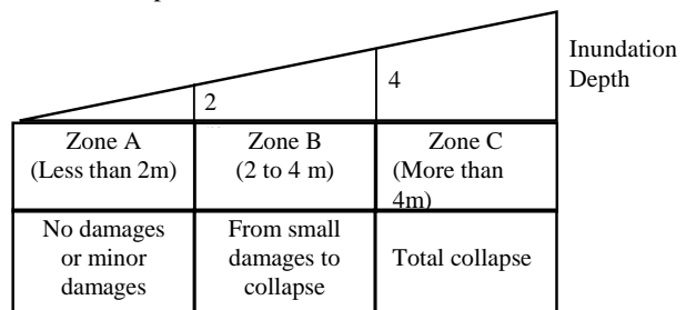
Fig. 6 Inundation depth and damages on wooden houses
