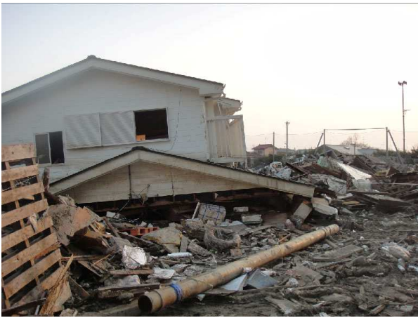
Fig. 8 Failure of the first floor
