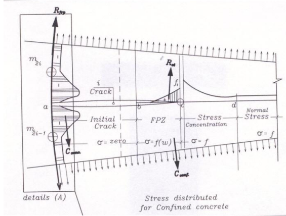
Fig. 8 Stress distribution, and resistance and acting forces position (Confined concrete model for meso/micro scale) [13]
