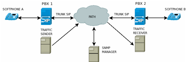
Fig. 4. Network testbed used for algorithm validation.
