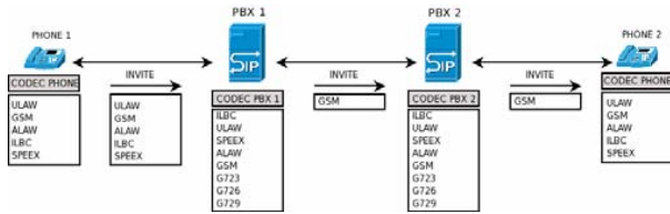
Fig. 1. Contents of the INVITE message during exchange between two SIP phones.
