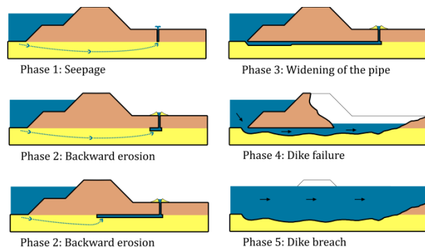
Fig. 1 Backward erosion piping [12]
