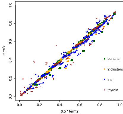
Fig. 7. The values of the second and third term are approximately equal for various data sets over the entire range of the parameters.
