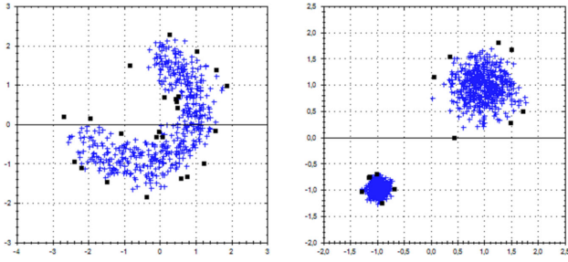
Fig. 9. Parameter tuning of SVDD on artificial two-dimensional data sets visualised in input feature space. (a) banana-shaped cluster and (b) two circular clusters following a Gaussian distribution with different densities (black squares: support vectors).
