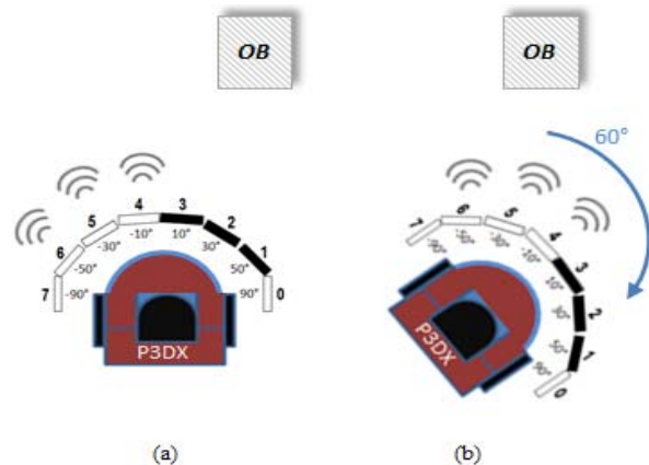
Fig. 8 Sonar sensors (1-3) as disabled (a); they are 'blind' to object OB . The Compensation Policy is used to establish that a 60° clockwise rotation (b), can allow the P3-DX robot to detect object OB
