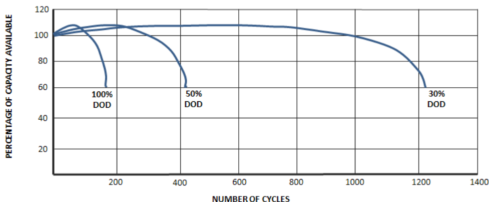
Fig. 1 Shows the DOD characteristics for the lead-acid battery used in the Pioneer 3-AT
