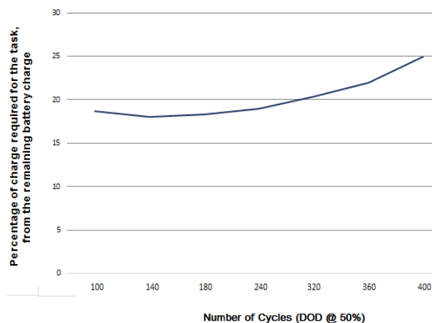
Fig. 4 The percentage charge required to complete a task at various battery cycle stages (DOD set at 50%)
