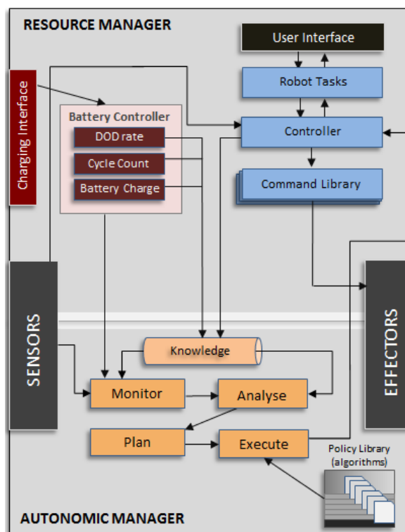
Fig. 3 Autonomic Battery Manager Model
