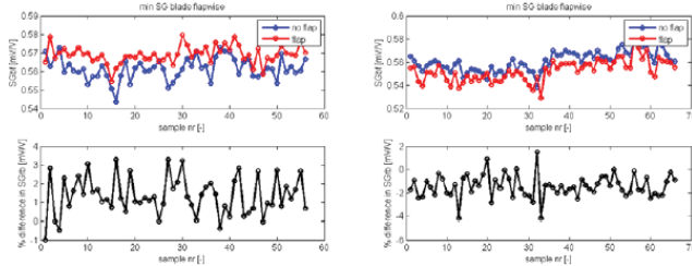
Fig. 11. Comparison of minimum flapwise bending moment at blade section root around tower passage between consecutive samples of no flap and flap activation (left: flap to max negative flap angle, right: flap to max positive flap deflection).
