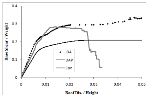
Fig. 3 Capacity curves for U1
